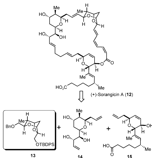
Scheme 3. Retrosynthetic analysis of (+)-sorangicin A.
