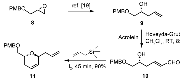
Scheme 1. Synthesis of 2,6-disubstituted-3,4-dihydropyran moiety using iodine as catalyst.
