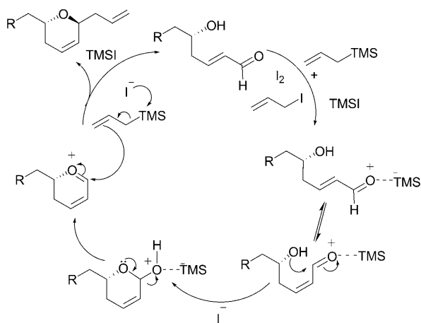
Scheme 2. Possible catalytic pathways for the formation of the product.
