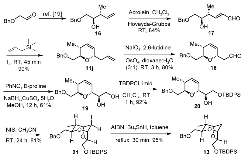
Scheme 4. Synthesis of C28-C37 fragment of (+)-sorangicin A.
