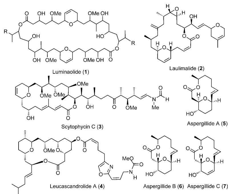
Figure 1. A few natural products bearing 2,6-disubstituted-3,4-dihydropyran moiety.
